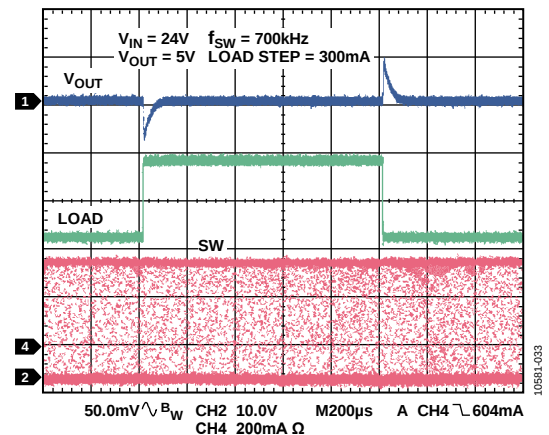
Figure 33. Load Transient Response, V_{IN} = 24\text{ V} , V_{OUT} = 5\text{ V} , f_{SW} = 700\text{ kHz} , Load Step = 300mA
