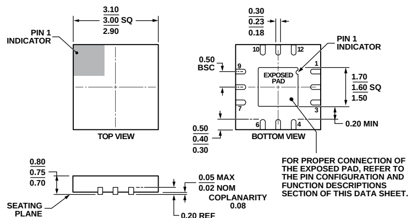
Figure 68. 12-Lead Lead Frame Chip Scale Package [LFCSP_WQ] 3 mm × 3 mm Body, Very Very Thin Quad (CP-12-6)
