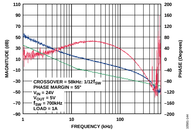
Figure 44. Magnitude and Phase vs. Frequency
