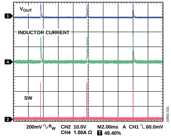
Figure 32. Hiccup Mode, V_{IN} = 24\text{ V} , V_{OUT} = 3.3\text{ V} , f_{SW} = 500\text{ kHz} , Output Short to PGND
