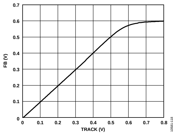
Figure 18. Tracking Range
