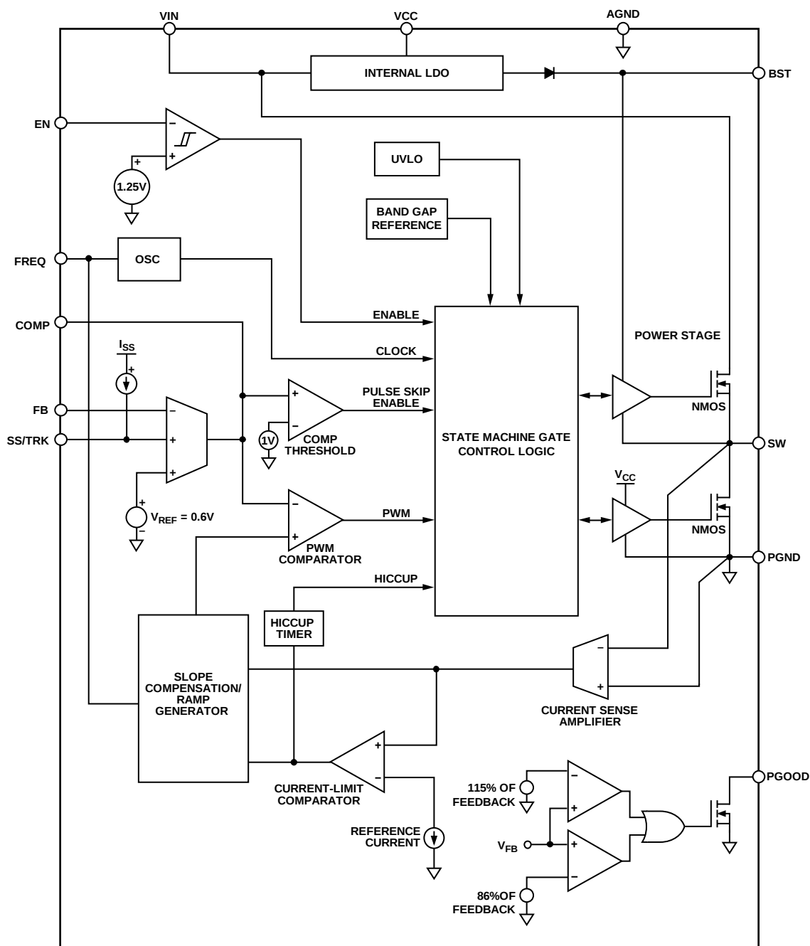
Figure 45. Block Diagram
