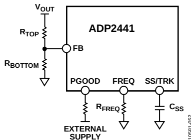
Figure 54. Voltage Divider
